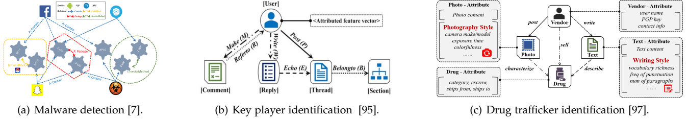
Fig. 9: The representative HGs in cybersecurity applications.
