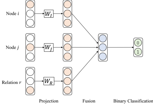
Fig. 4: The architecture of HIN2vec. Through the parameter matrices \mathbf{W}_I , \mathbf{W}_J and \mathbf{W}_R , the one-hot vectors of node i , node j and relation r are projected into dense vectors. And these three vectors are fused by a neural network to predict whether node i and j are connected by relation r .
