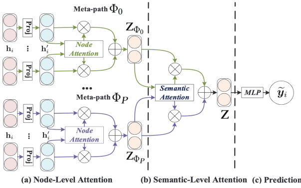
Fig. 5: The architecture of HAN [15]. The whole model can be divided into three parts: Node-Level Attention aims to learn the importance of neighbors' features. Semantic-Level Attention aims to learn the importance of different meta-paths. Prediction layer utilizes the labeled nodes to update the node embeddings.
