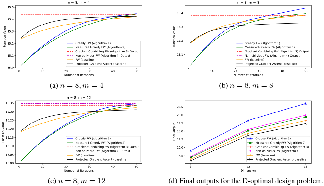
Figure 3: Plots 3a , 3b , and 3c correspond to the quadratic programming experiment from Section 4.2.1 . Plot 3d pertains to the D-optimal experimental design problem from Section 4.2.2 .
