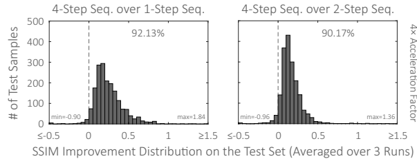
Figure 7: Histograms of pair-wise SSIM comparison on all 1,851 test images with a different number of sequential steps ( T ), using 2D point sampling with a 4\times acceleration factor. The relative error between the 4-step and 1-step (left) or 2-step (right) demonstrates that additional sequential steps help to boost performance, but with diminishing returns as T increases.
