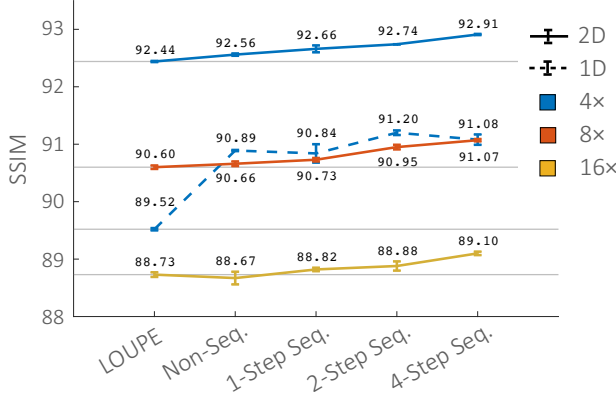
Figure 6: Comparison between our sequential model and the LOUPE model on the fastMRI knee test set. Our sequential model outperforms LOUPE for all acceleration ratios with an improvement comparable to 25% of the benefit of doubling the number of \kappa -space measurements. The performance of our sequential model in the 1D line sampling case significantly outperforms LOUPE but plateaus after 2 sequential sampling steps, possibly due to the restricted action space of 1D line sampling.
