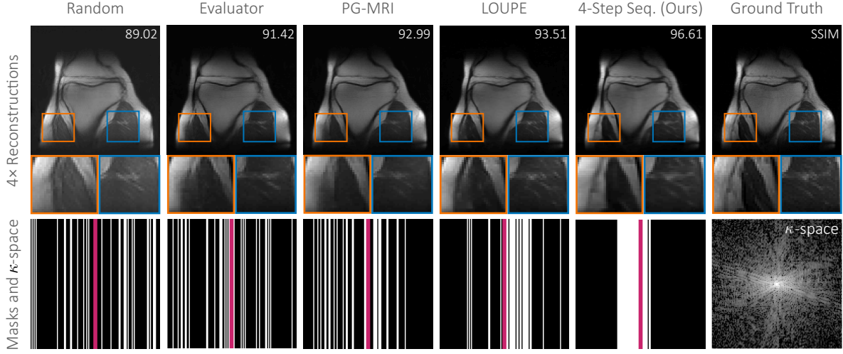
Figure 4: Visualizations of example reconstructions with an 4 \times acceleration for 1D line sampling. Two zoomed-in image patches are shown along with the cumulative \kappa -space measurements selected by each policy. Our sequential approach often provides more accurate reconstructions with detailed local structures. More visualizations are included in the Appendix D.
