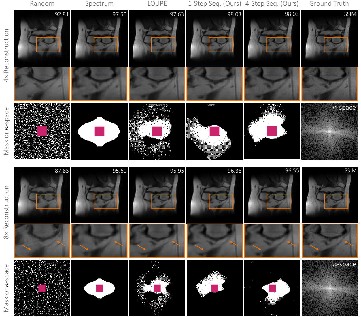
Figure 14: Visualizations of the reconstructions of the 1355 th test sample with an acceleration factor of 4\times (top) and 8\times (bottom) for 2D point sampling. A zoomed-in image patch is shown along with the cumulative \kappa -space measurements selected by each policy. Orange arrows point out the regions where our sequential approach provides more accurate detailed local structures.
