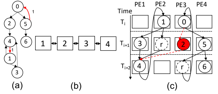
Fig. 1. a) DFG of an application loop. (b) A 1x4 CGRA target architecture. (c) Failure to map node 2 by GraphMinor
