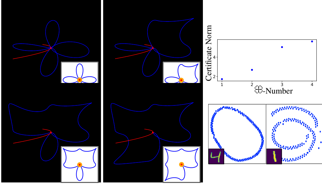
Figure 2: The clover-number—theory and practice. Left: We generate a parametric family of space curves with fixed maximum curvature and length, but decreasing clover-number, by reflecting ‘petals’ of a clover about a circumscribing square. We set \mathcal{M}_+ to be a fixed circle with large radius that crosses the center of the configurations, then rescale and project the entire geometry onto the sphere to create a two curve problem instance. In the insets, we show a two-dimensional projection of each of the blue \mathcal{M}_- curves as well as a base point x \in \mathcal{M}_+ at the center (also highlighted in the three-dimensional plots). The intersection of \mathcal{M}_- with the neighborhood of x denoted in orange represents the set whose covering number gives the clover-number of the configuration (see (2.2)). Top right: We numerically generate a certificate for each of the four geometries at left and plot its norm as a function of clover-number. The trend demonstrates that increasing clover-number correlates with increasing classification difficulty, measured through the certificate problem: this is in line with the intuition we have discussed. Bottom right: t-SNE projection of MNIST images (top: a “four” digit; bottom: a “one” digit) subject to rotations. Due to the approximate symmetry of the one digit under rotation by an angle \pi , the projection appears to nearly intersect itself. This may lead to a higher clover-number compared to the embedding of the less-symmetric four digit. For experimental details for all panels, see Appendix A.
