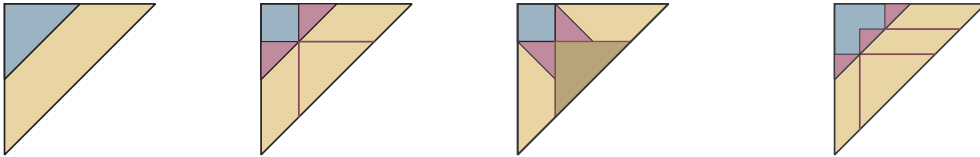
FIGURE 10. Making two smaller slim diagrams out of thick ribbon \tau_k , where k is even. Same with three slim diagrams.
