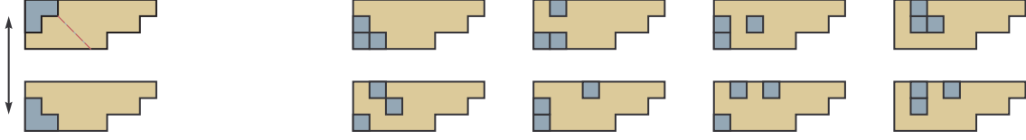
FIGURE 9. Slim skew shape \lambda/\mu , where \lambda = (9, 8, 6) , \mu = (2, 1) , and the set \mathcal{E}^\diamond(\lambda/\mu) of flipped excited diagrams.
