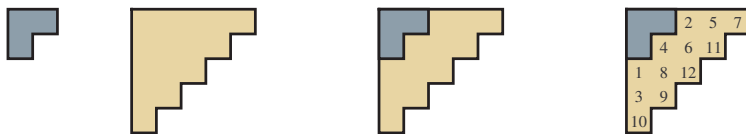
FIGURE 1. Staircases \delta_3 and \delta_6 , thick ribbon \tau_3 = \delta_6/\delta_3 , and a standard Young tableau of shape \tau_3 .
