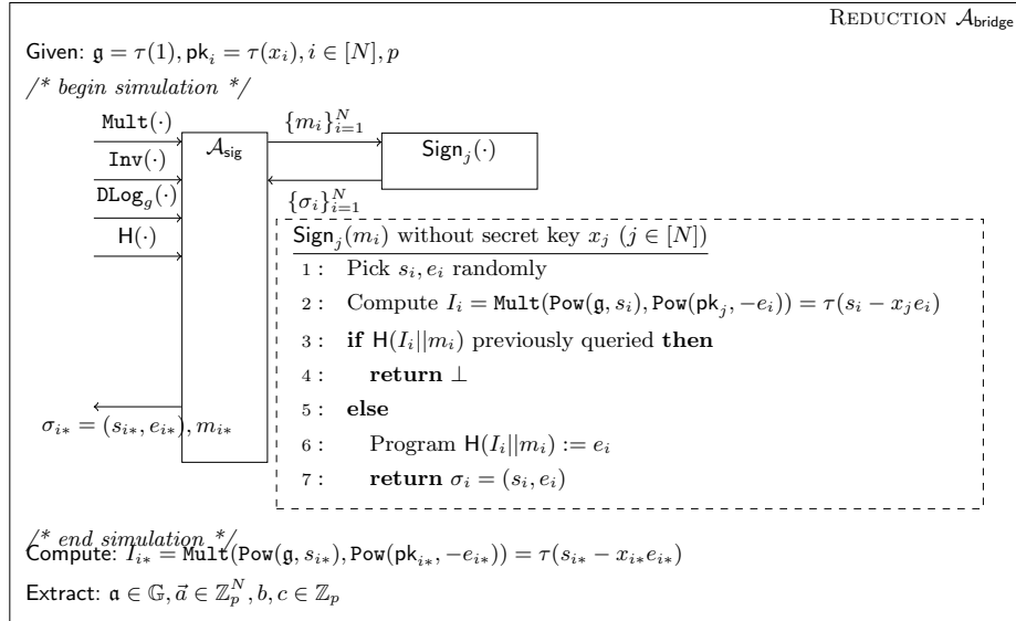
Figure 2. A reduction to the \text{BridgeChal}_{\mathcal{A}_{\text{bridge}}}^{\tau, N}(k) attacker \mathcal{A}_{\text{bridge}} from the short Schnorr signature attacker \mathcal{A}_{\text{sig}} .
