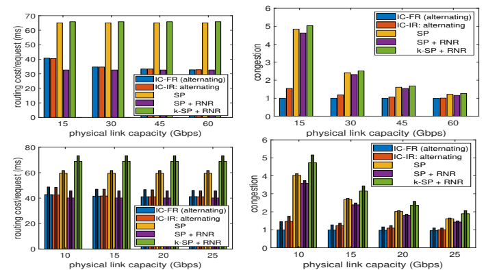
Fig. 8. General case under varying link capacity: first row – synthetic simulation, second row – trace-driven simulation (light: true demand; dark: predicted demand).
