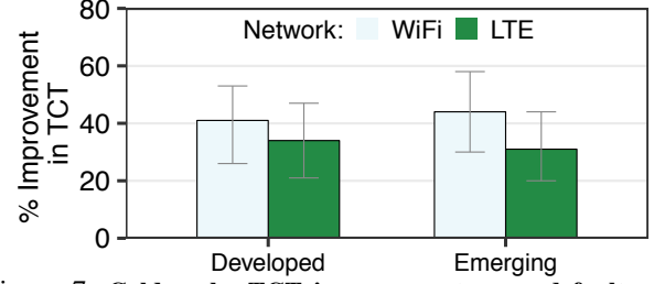
Figure 7: Cold cache TCT improvements over default page loads. Bars list medians, with error bars for 25-75th percentiles.
