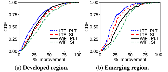
Figure 8: Distributions of cold cache per-page improvements with Horcrux vs. default page loads.
