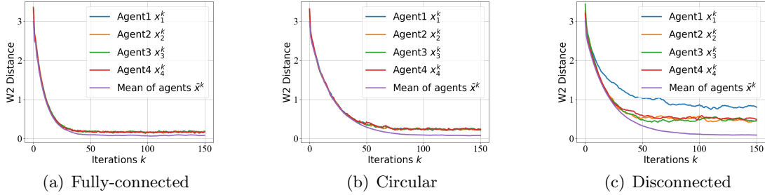
Figure 3: Performance of DE-SGHMC method for Bayesian regression on different network structures. The stepsize \eta and the friction coefficient \gamma are tuned to the dataset where we take \eta = 0.1 and \gamma = 7 .
