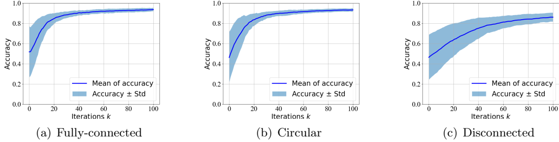
Figure 7: The plots show the accuracy over the data set versus number of iterations for the DE-SGLD method on different network structures over Breast Cancer data set. Figures are based on one randomly picked agent. Here, the stepsizes are chosen as \eta = 0.0008 . We use batch size b = 32 in the experiments.
