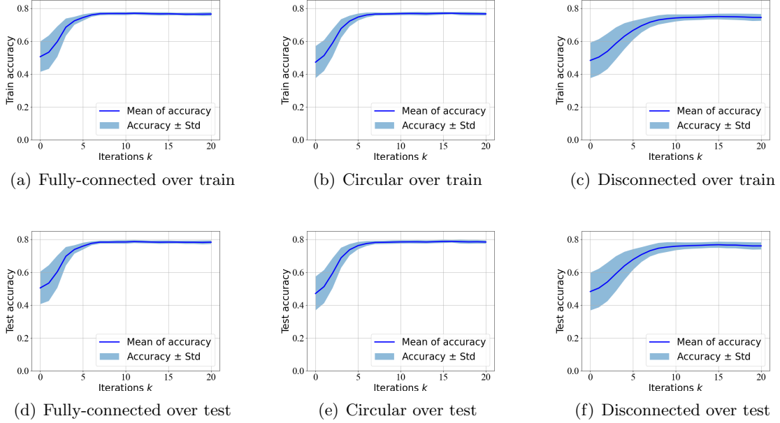
Figure 10: The plots show the accuracy over the data set versus number of iterations for the DE-SGHMC method on different network structures over training data and test data from the Telescope data set. Figures are based on one randomly picked agent. Here, the stepsize \eta and the friction coefficient \gamma are tuned to the data set where we take \eta = 0.07 , \gamma = 5 . We use batch size b = 100 in the experiments.
