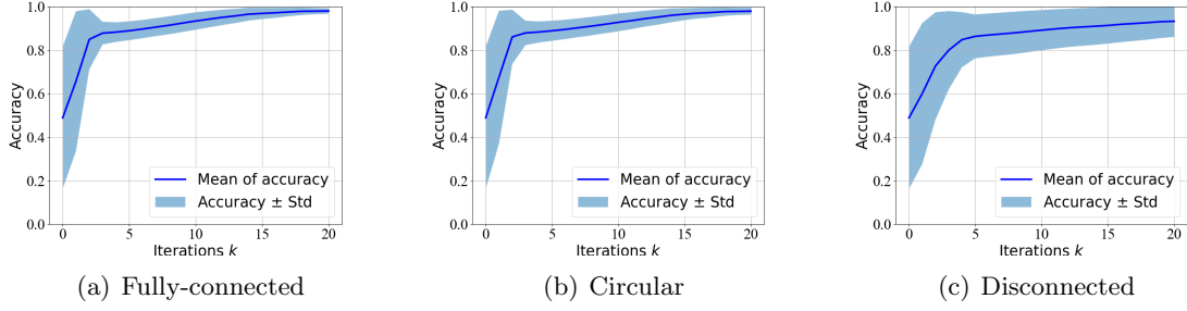
Figure 6: The plots show the accuracy over the data set versus number of iterations for the DE-SGHMC method on different network structures. Figures are based on one randomly picked agent. Here, the stepsize \eta and the friction coefficient \gamma are tuned to the dataset where we take \eta = 0.02 and \gamma = 30 . We use the stochastic gradient with batch size b = 32 in the experiments.
