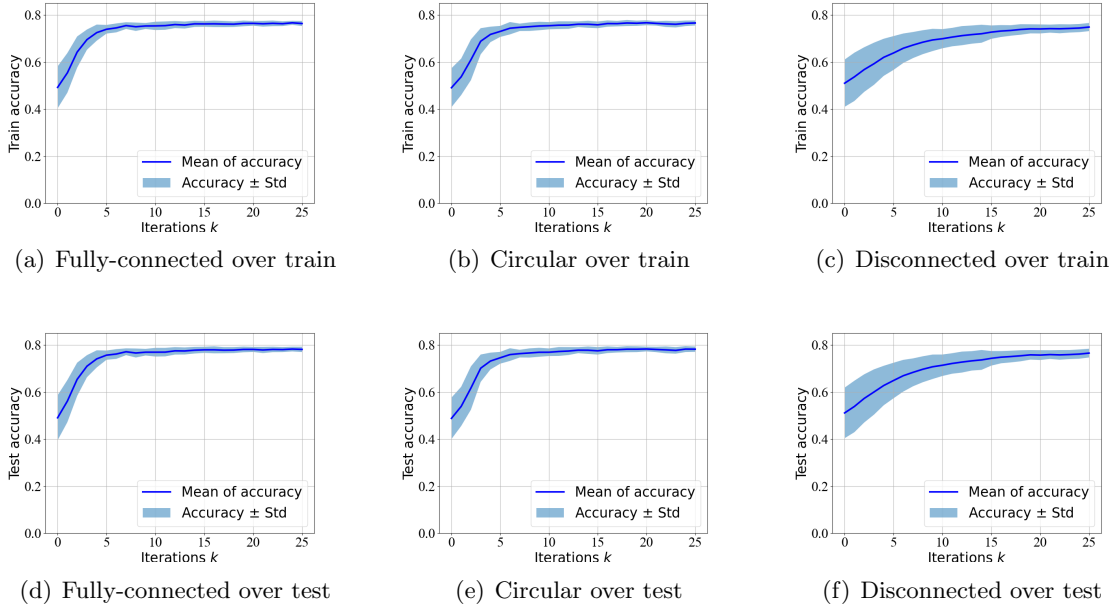
Figure 9: The plots show the “distribution of the accuracy over the data set” versus number of iterations for the DE-SGLD method on different network structures over the training data and the test data of Telescope data set. Figures are based on one randomly picked agent. Here, the stepsizes are chosen as \eta = 0.008 . We use batch size b = 100 in the experiments.
