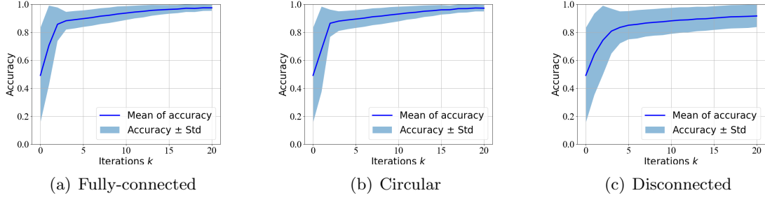
Figure 5: The plots show the the accuracy over the data set versus number of iterations for the DE-SGLD method on different network structures. Figures are based on one randomly picked agent. Here, the stepsizes are tuned to the dataset where we take \eta = 0.0003 . We use the stochastic gradient with batch size b = 32 in the experiments.
