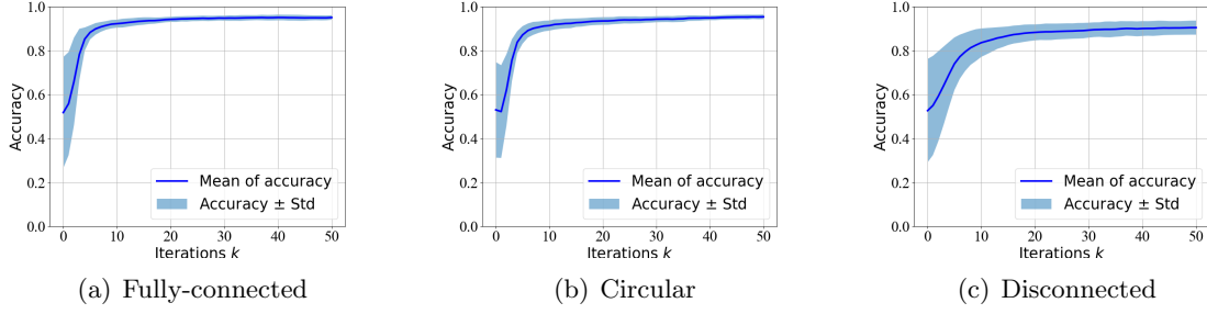
Figure 8: The plots show the accuracy over the data set versus number of iterations for the DE-SGHMC method on different network structures over Breast Cancer data set. Figures are based on one randomly picked agent. Here, the stepsize \eta and the friction coefficient \gamma are well tuned to the data set so that we take \eta = 0.05 , \gamma = 10 . We use batch size b = 32 in the experiments.
