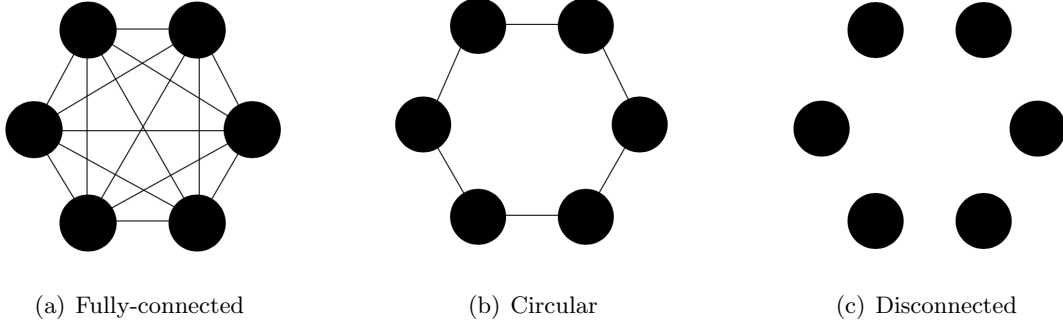
Figure 1: Illustration of the network architectures.
