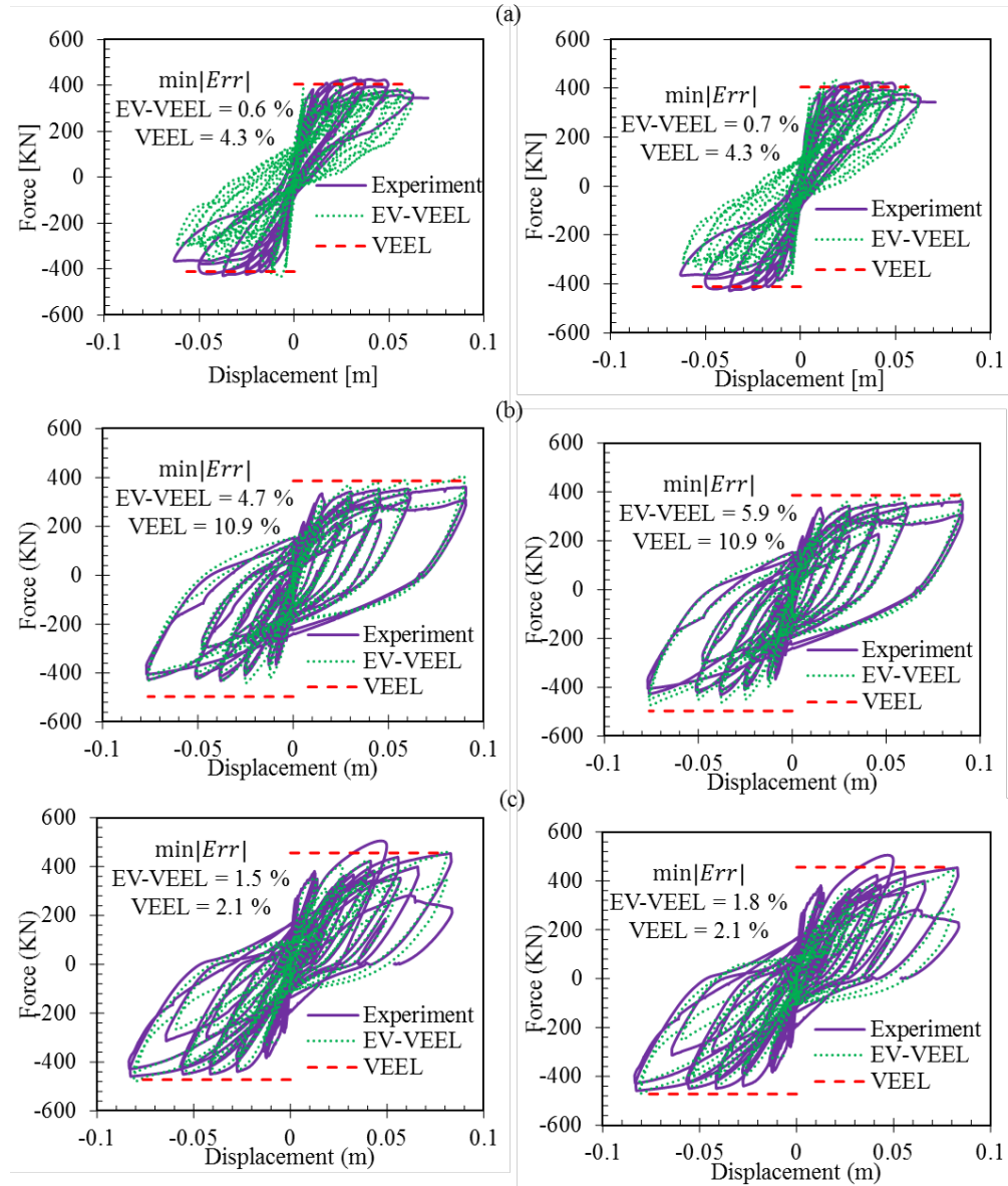
Figure 6: Comparison between the accuracy of Model I (left column), Model II (right column), and VEEL for the walls WSH5 and TUB: (a) results for WSH 5; (b) results of north-south direction loading for TUB; (c) results of east-west direction loading for TUB.
