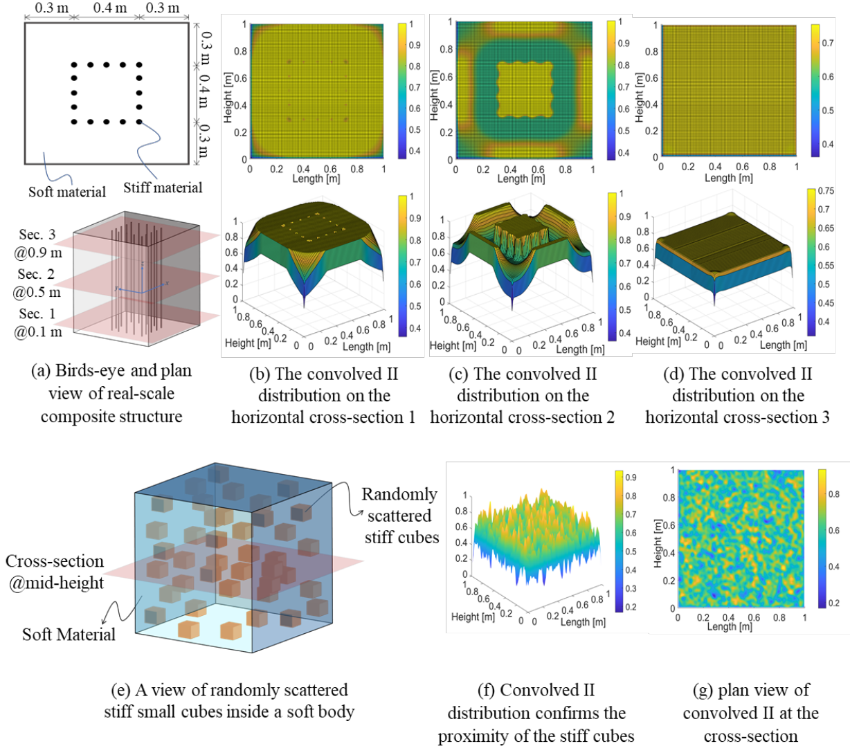
Figure 3: Examples of (a-d) II-based perception of stiff objects, BC's, and (e-g) heterogeneity.
