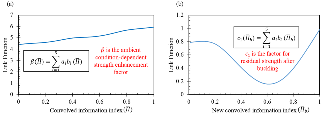
Figure 8: Material coefficients through an LF: (a) an example of material coefficient that affects the strength of the brittle material; (b) an example of material coefficient that affects the buckling of the reinforcement steel.
