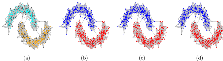
Figure 4: True density (column 1), PPR (column 2), minimum normalized cut (column 3) and estimated density (column 4) clusters for two-moons with 10 dimensional noise. Seed node for PPR denoted by a black cross.
