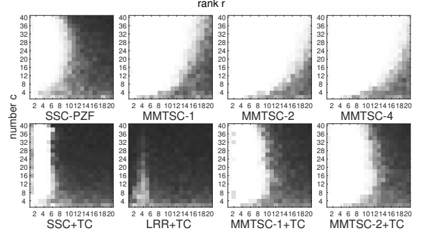
Figure 3: Phase transitions for different rank r and number of subtensors per cluster c ( p = 0.5 ).
