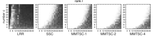
Figure 4: Phase transitions for different rank r and number of subtensors per cluster c ( p = 1 ).
