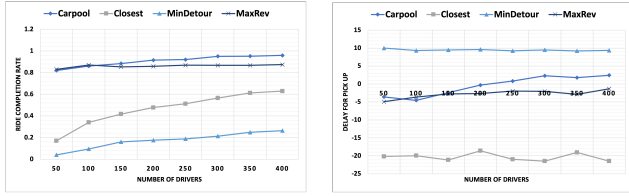
(a) Route recommendations lead to almost optimal ride completion. (b) Route recommendations lead to minimal pickup delays.
