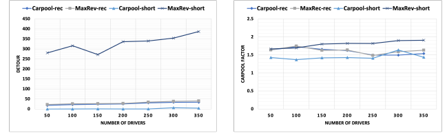
(c) Detour flexibility is leveraged only when needed. (d) Carpool factor is almost at the maximum of 2 passengers per driver.
