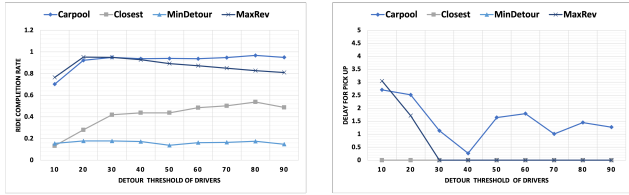
(a) Following recommended rides and routes allow for almost optimal ride completion rate. (b) Almost no delays with increased detour.
