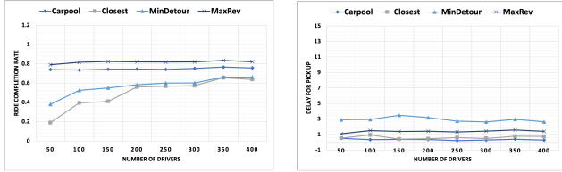
(c) Shortest paths don't reach optimal completion rates. (d) Shortest paths lead to an increase in pickup delays.
