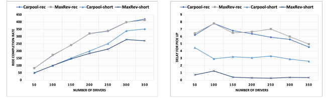
(a) Completion rate increases. (b) Delays are minimally affected.
