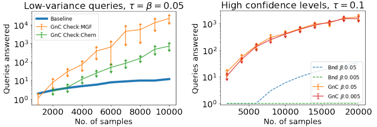
Figure 4: Left: Gain in performance for GnC Gauss by using Lemma 3.1 for HoldoutTol (“GnC Check:MGF”), as compared to using Lemma C.9 (“GnC Check:Chern”). Right: Performance of GnC Gauss (“GnC”), and the best Gaussian bounds (“Bnd”), for \beta \in \{0.05, 0.005\} .
