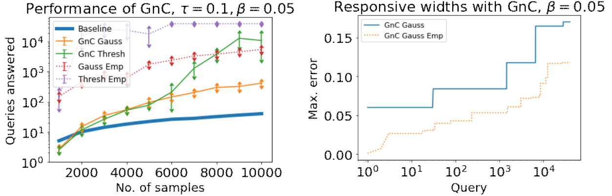
Figure 5: Left : Performance of GnC with Gaussian (“GnC Gauss”), and Thresholdout (“GnC Thresh”) mechanisms, together with their empirical error. Right : The accuracy of GnC with Gaussian guesses provides “responsive” confidence interval widths that closely track the empirical error incurred by the guesses of the Gaussian mechanism (“GnC Gauss Emp”).
