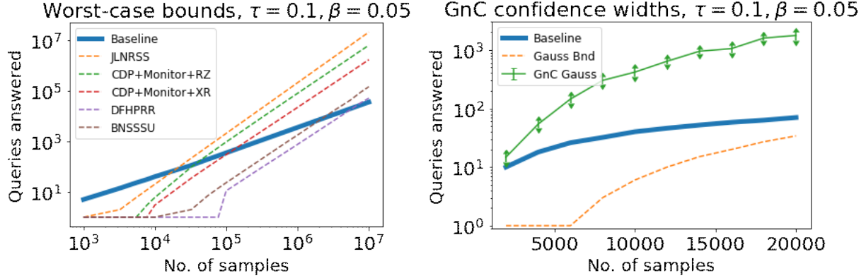
Figure 1: Left : Comparison of various worst-case bounds for the Gaussian mechanism with the sample splitting baseline. ‘DFHPRR’ and ‘BNSSSU’ refer to bounds given in prior work (Dwork et al. [2015d], Bassily et al. [2016]). The other lines plot improved worst-case bounds derived in this paper, whereas ‘JLNRSS’ refers to bounds in subsequent work (Jung et al. [2019]). (See Section 2 for the full model and parameter descriptions.) Right : Performance of Guess and Check with the Gaussian mechanism providing the guesses (“GnC Gauss”) for a plausible query strategy (see Section 3.1), compared with the best worst-case bounds for the Gaussian mechanism (“Gauss Bnd”), and the baseline.
