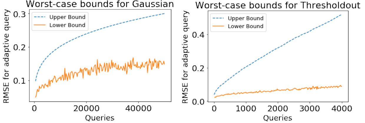
Figure 2: Worst-case upper (proven) and lower RMSE bounds (realized via the single-adaptive query strategy) with n = 5,000 for Gaussian (left) and Thresholdout (right).
