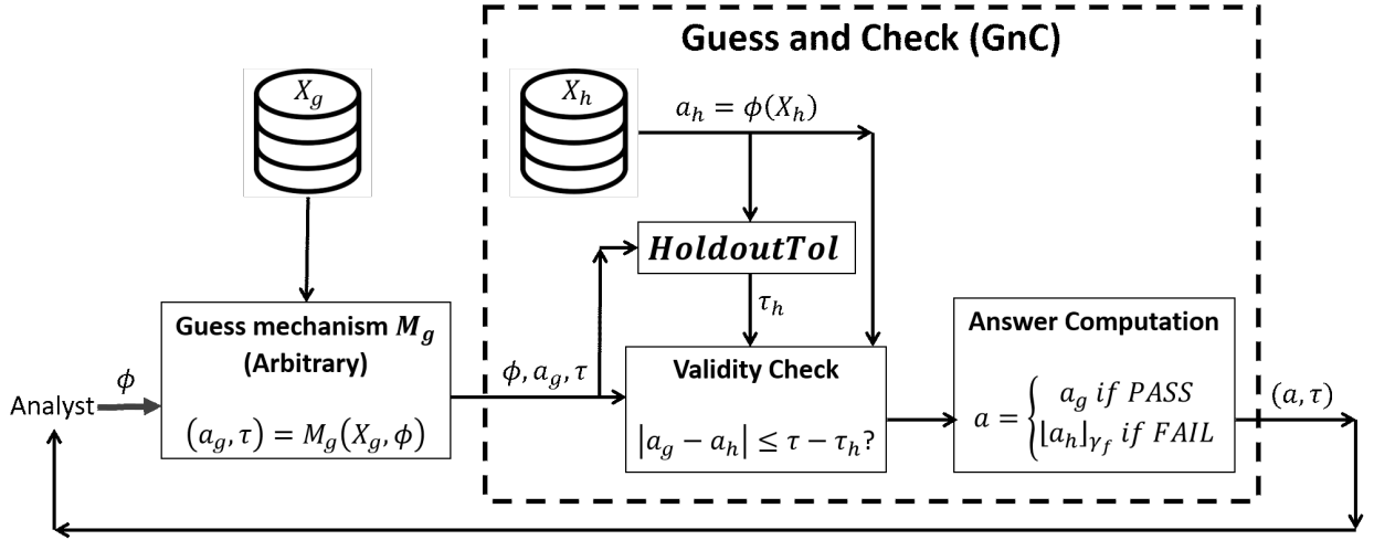
Figure 3: A schematic of how query \phi is answered via our Guess and Check (GnC) framework. Dataset X_g is the guess set randomly partitioned by GnC. The dotted box represents computations that are privileged, and are not accessible to the analyst.
