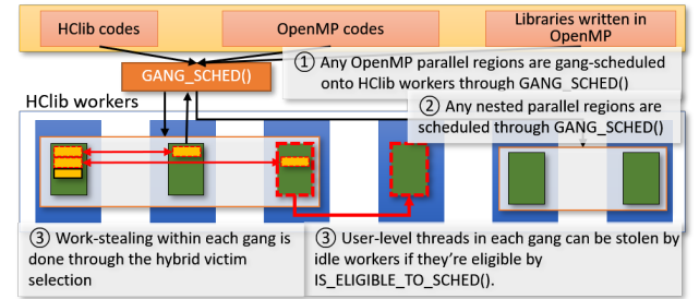
Figure 3. Implementation of Integrated HClb and OpenMP runtime
