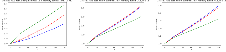
Figure 1: Blue is Algorithm 2, green is Algorithm 1, and red is the algorithm of [11]. We show the median of 5 trials, with error bars showing the smallest and largest relative errors across those trials.
