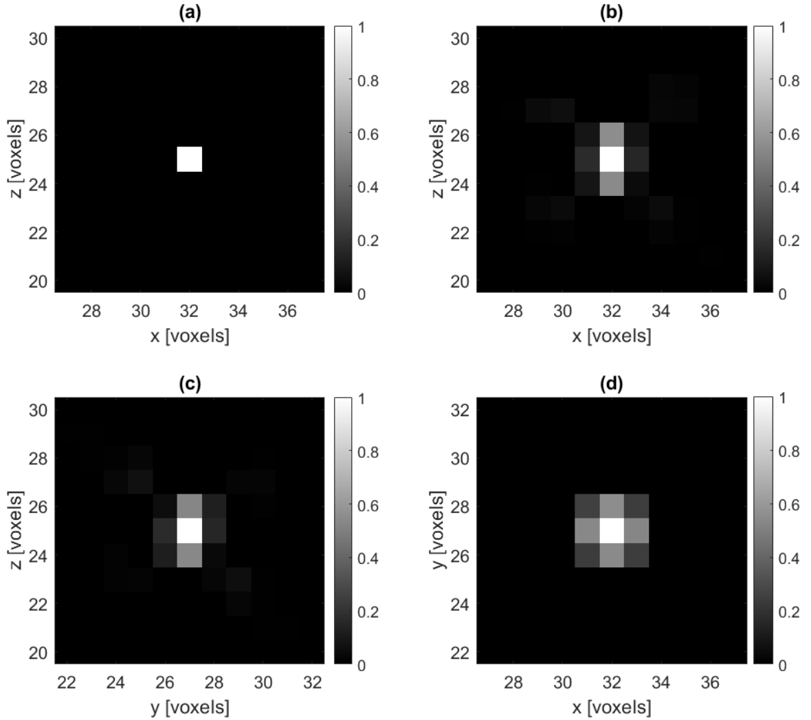
Figure 3. (a) A cross-section of the ground truth impulse IPD and (b,c,d) cross-sections of a no-noise reconstruction of the impulse IPD. Here we use regularization parameter \lambda = 2.5 \cdot 10^{-4} in (6).
