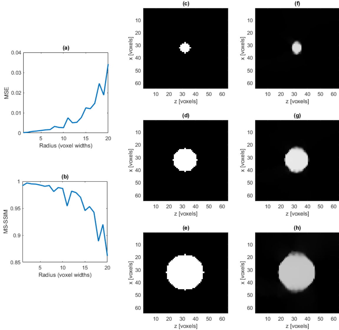
Figure 6. Average MSE (a) and average MS-SSIM (b) of the reconstructed cylinder IPD with varying radius, averaged over five trials for each radius value considered. A cross section of the ground truth cylinder with radius of five (c), ten (d) and fifteen (e) voxel widths and a cross section of the reconstruction of the same cylinder, respectively (f,g,h). Each cylinder considered is orthogonal to the xz -plane.
