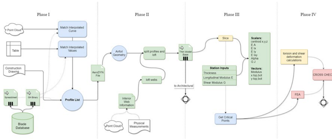
Figure 1. Logic flow diagram of the Blade Machine Phases.
