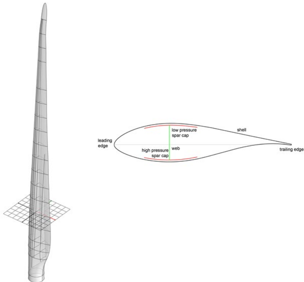
Figure 4. Thin model output from Phase II showing interior web and spar cap information.
