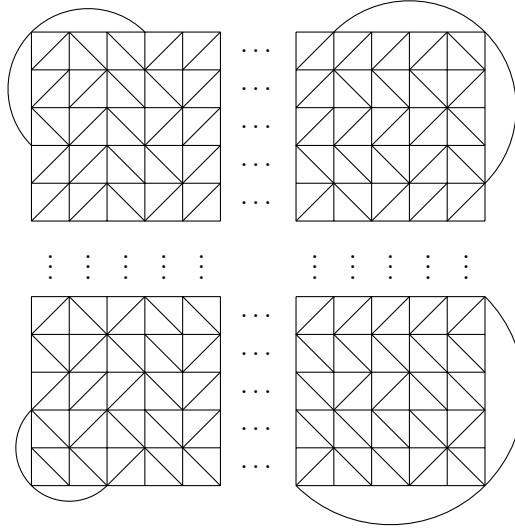
Figure 1: An example of one of the graphs from our family \mathcal{B} .
