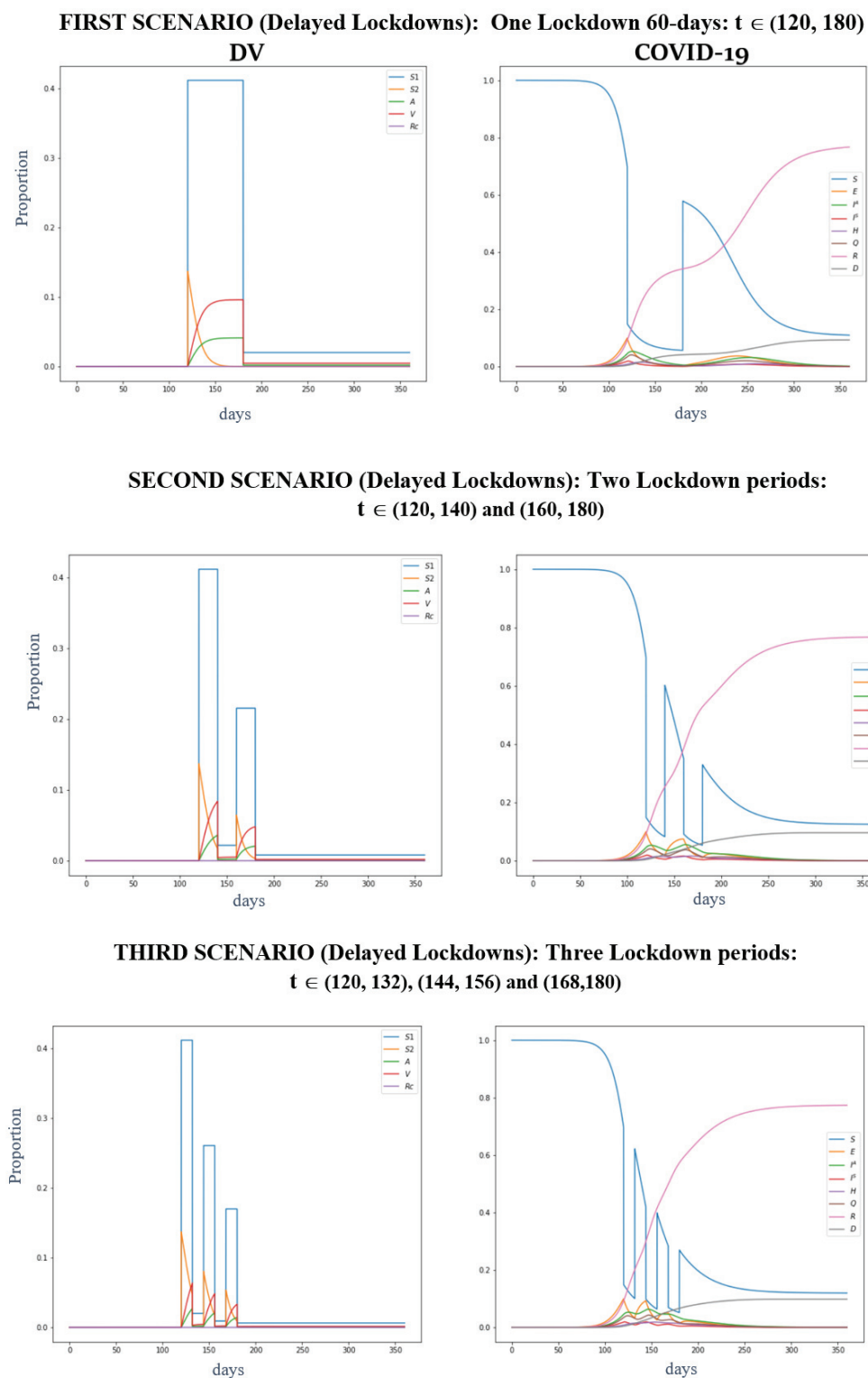
Figure 4. Model 1 simulation results as in Table 4.
