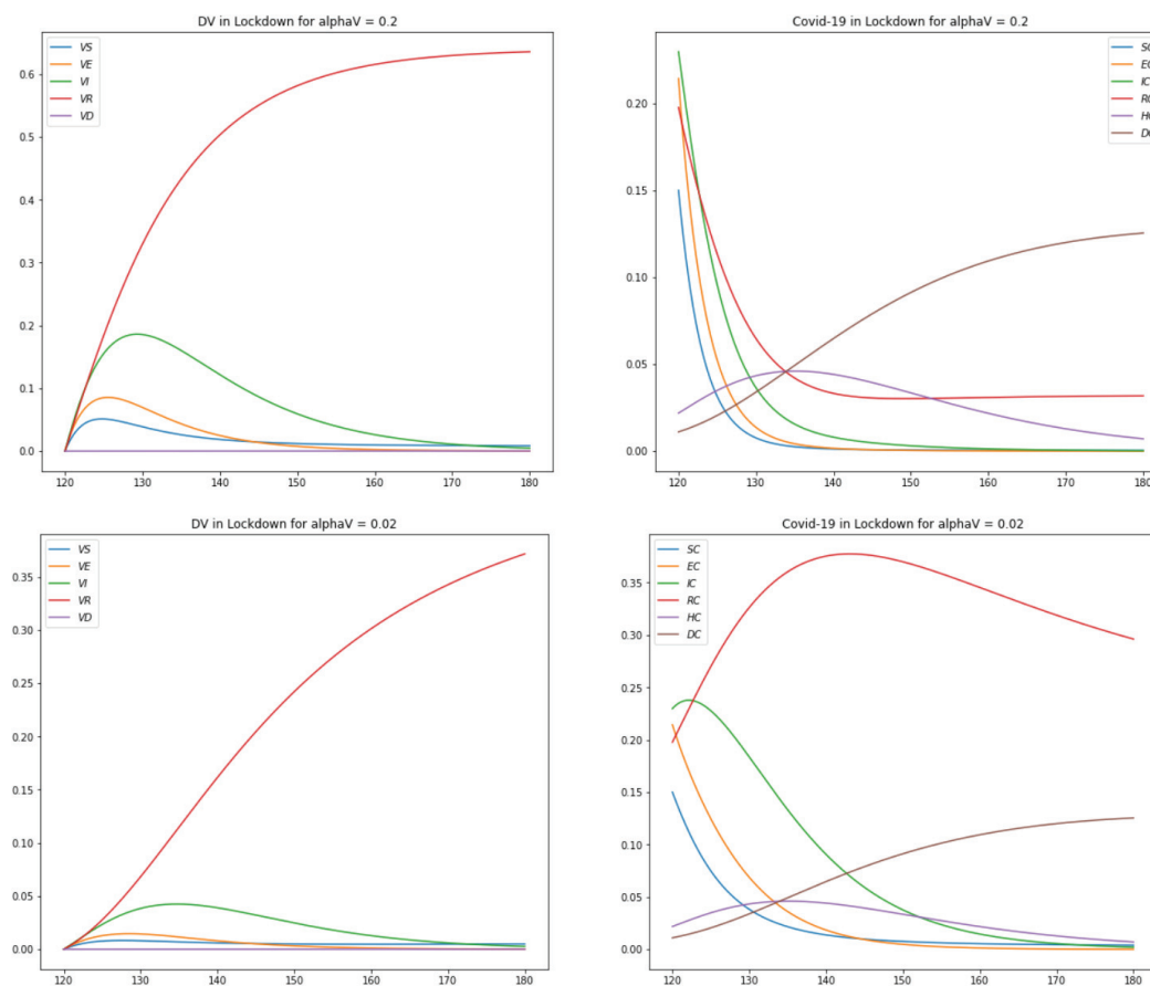
Figure 5. Model 2 Results for high and low \alpha^V .
