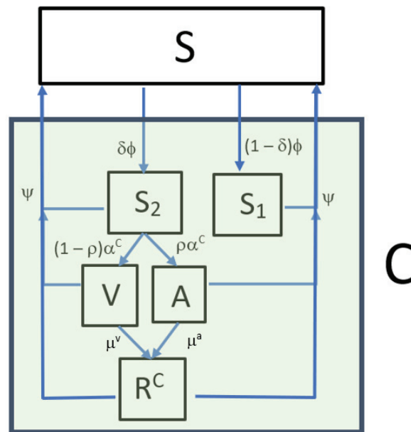
Figure 2. Model 1 flow diagram of Model 1 DV-confinement compartment.
