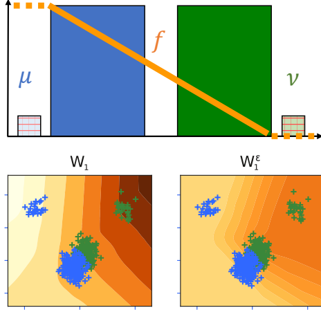
Figure 3: Optimal potentials: (top) 1D densities plotted with their optimal potential for the W_1^\varepsilon dual problem; (bottom) contour plots for optimal dual potentials to W_1 and W_1^\varepsilon between 2D Gaussian mixtures. Observe how optimal potentials for the robust dual are flat over outlier mass.
