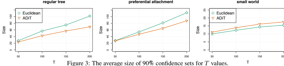
Figure 3: The average size of 90% confidence sets for T values.
