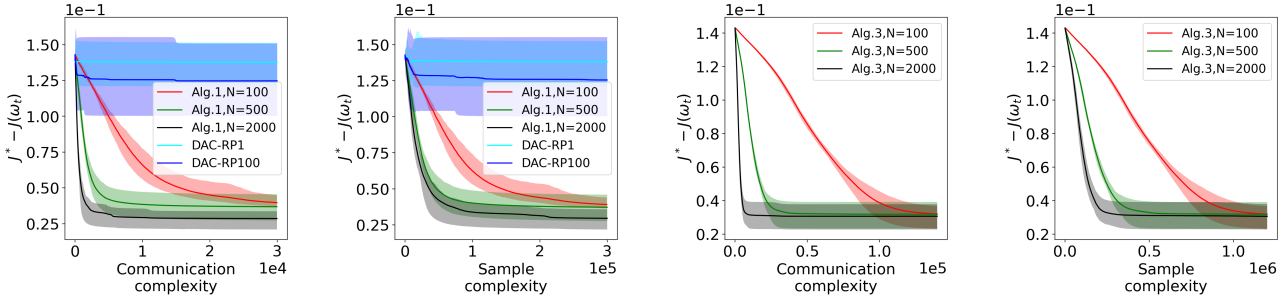
Figure 3: Comparison of optimality gap J^* - J(\omega_t) among decentralized AC-type algorithms in fully connected network.
