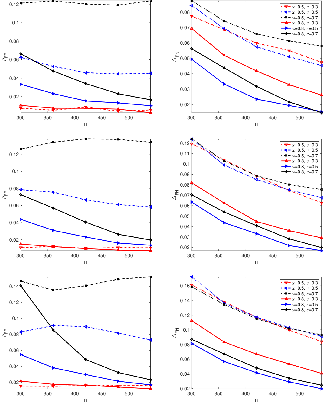
Figure 3: The false positive rates \rho_{FP} (left panels) and the rates \Delta_{FN} (right panels) for K = 4 (top), K = 5 (middle) and K = 6 (bottom) clusters. The rates are evaluated over 100 simulation runs. The number of nodes ranges from n = 300 to n = 540 with the increments of 60. Dashed lines represent the results for \omega = 0.5 and solid lines represent the results for \omega = 0.8 ; \sigma = 0.3 (red), \sigma = 0.5 (blue) and \sigma = 0.7 (black).
