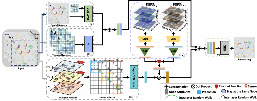
Figure 1: TAMP-S2GCNets consists of 5 components: (I) Spatial graph convolutional layer on \mathcal{G}_t extracts spatial information at time t (see Eq. 5). (II) Feature transformation (FT) learns representation of the spatio-temporal data \mathcal{X}^T over a sliding window of size T (see Eq. 1). (III) Supragraph convolutional module captures joint spatio-temporal dependencies in \mathcal{X}^T (see Eq. 4). (IV) Detailed architecture of the DEPSRL module (see Eqs. 6 and 7), where the DEPS with different types of multifiltrations can be learned by a CNN base model and global pooling mechanism. Here DEPS allows us to learn the intrinsic graph structure both across multiple geometric dimensions and across time. (V) The learned spatio-temporal dependencies are passed into GRU layer (see Eq. 8) for multi-step forecasting. Note that the whole model can be trained in an end-to-end fashion.
