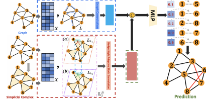
Figure 2: The architecture of BScNets. BScNets consists of graph convolution (upper row) and Hodge-style adaptive block convolution module (lower row). Each convolution layer/module contains the node feature matrix \mathbf{X} and a Laplacian/operator (i.e., normalized Laplacian \tilde{\mathbf{L}} and adaptive Hodge Laplacian based operator \mathbb{L}_2^B for upper and lower parts respectively). Lower row presents the relation modeling between (a) Hodge Laplacian \mathbf{L}_{k_1} describing diffusion from edge to edge through nodes and (b) Hodge Laplacian \mathbf{L}_{k_2} describing diffusion from edge to edge through triangles. Symbol \odot represents concatenation.
