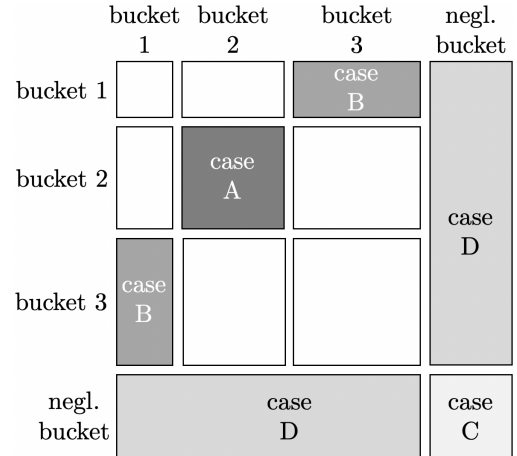
Figure 1: Partition of \sigma into blocks corresponding to buckets, relevant submatrix for each case highlighted in gray.
