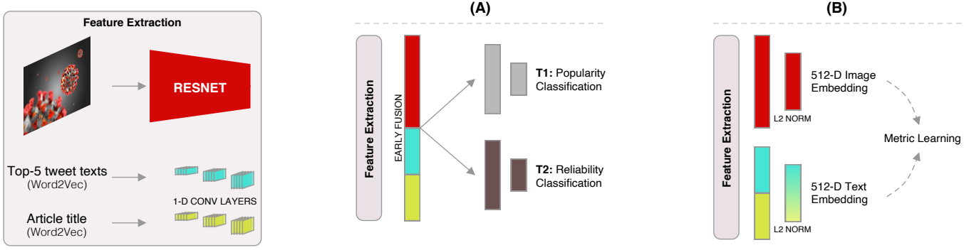
Figure 2: (A) Multi-task architecture for multi-modal popularity and reliability classification. Features from both modalities extracted through convolutional layers are fused to perform both tasks simultaneously. (B) Cross-modal relation modeling. Visual and text features from the same article are embedded in a metric space to understand how image-text composition varies in un/reliable articles. Note: The feature extraction module does not share weights between the two architectures.
