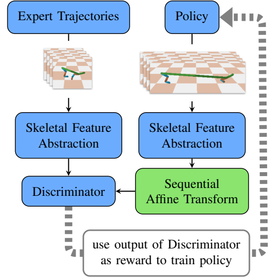
Fig. 1: A high level overview of the proposed technique, SILEM. The policy and discriminator are learned through a mini-max game as in prior AIL algorithms, while the sequential affine transform is learned by backpropagating through the discriminator (Algorithm 1).
