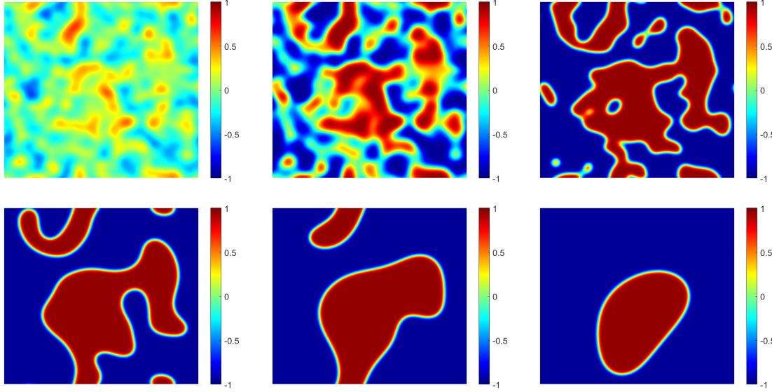
Fig. 8 Simulated phase structures at t = 4, 6, 10, 30, 100 , and 300 , respectively (left to right and top to bottom) by the sESAV2 scheme with \tau = 0.01 and \kappa = 8.02 for the coarsening dynamics of the Flory–Huggins potential case.
