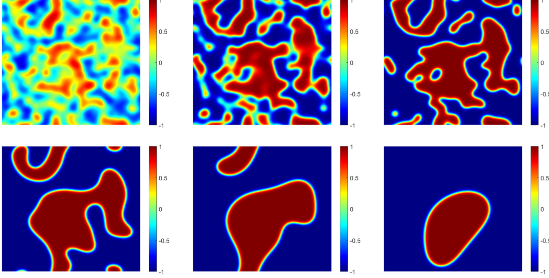
Fig. 6 Simulated phase structures at t = 4, 6, 10, 30, 100 , and 300 , respectively (left to right and top to bottom) by the sESAV2 scheme with \tau = 0.01 and \kappa = 2 for the coarsening dynamics of the double-well potential case.
