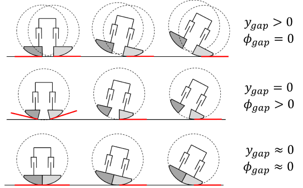
Fig. 3. Different foot geometries used in simulation and experiments. Top row: Nonconcentric feet with a gap. Middle row: Concentric feet with a gap. Bottom row: Feet with a negligible gap. Red lines indicate the contact point and angle of the surface of the foot at the contact point.
