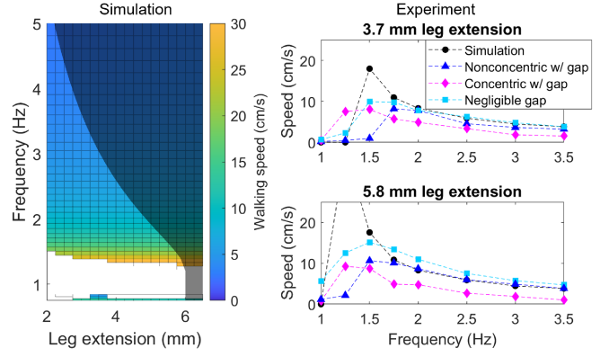
Fig. 4. Forward walking speed simulation (left) and experimental (right) results from sagittal plane model at different frequencies and amplitudes of oscillations. For the simulation: White region is unsuccessful walking and the dark region indicates the actuation limit of the servo used on the physical robot. Experimental trends follow simulation predictions: the highest walking speed is achieved between 1.25 and 1.5 Hz, and the speed gradually decreases with increasing frequency above that point.
