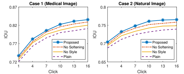
Figure 8: Ablation study. Results are reported in terms of refined segmentation (IoU) on two datasets with respect to the number of interactions.
