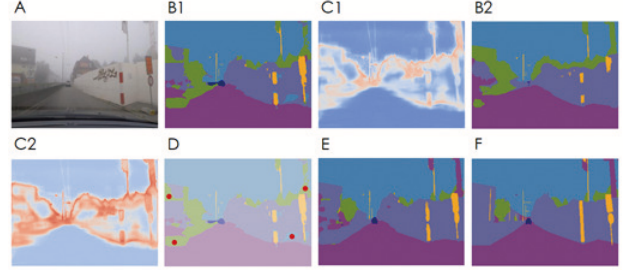
Figure 2: An illustrative example. Given an image (A), the model applies the first-level information filtering and makes an initial prediction (B1) with predictive entropy visualized in (C1). Without information filtering, the segmentation (B2) is worse, and the corresponding entropy (C2) is higher. After that, the user annotates a few pixels (D) highlighted in red, and the model applies the second-level information filtering and refines segmentation (E). Ground-truth is given in (F).
