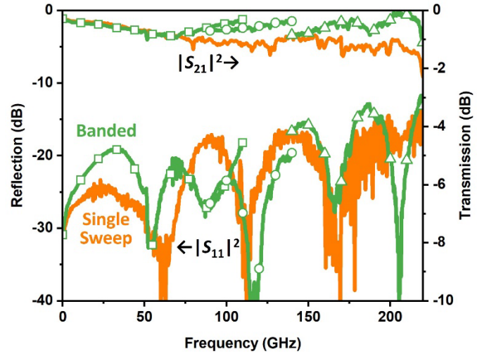
Fig. 4. S_{11} and S_{21} measured on an 1277-μm-long GCPW in a single sweep from 0.1 to 220 GHz or in bands of 0.1–110 GHz ( \square ), 90–140 GHz ( \circ ), and 140–220 GHz ( \triangle ).
