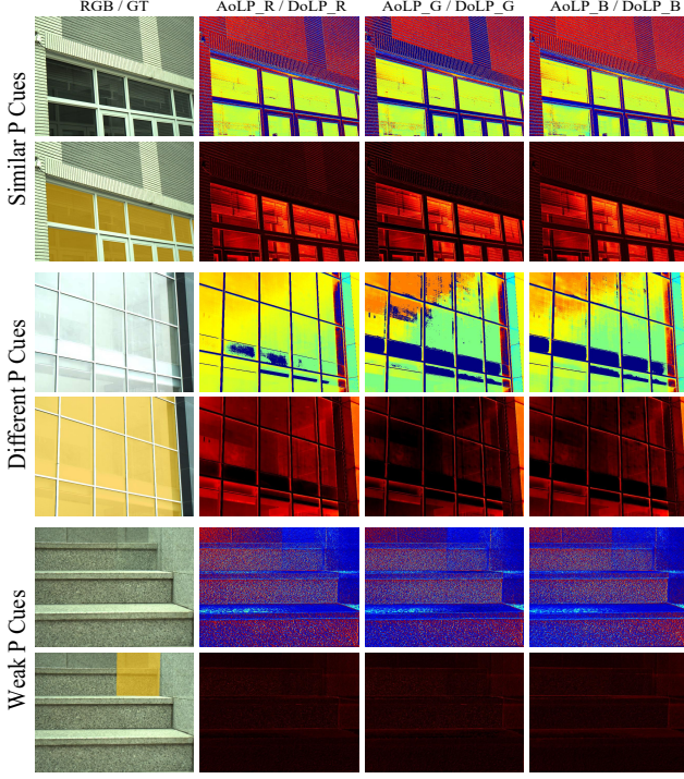
Figure 2. RGBP-Glass Examples. For each exemplar we show two rows, with in the first column the RGB intensity (top) and reference glass segmentation (bottom), and in the last three columns the polarization measurements for the red, green, and blue channels, respectively (top: AoLP, bottom: DoLP). The top exemplar exhibits clear glass cues in both RGB and polarization. The middle exemplar features weak intensity cues, but a strong polarization cues in the red channel. The bottom exemplar does not show strong cues in either RGB or polarization.
