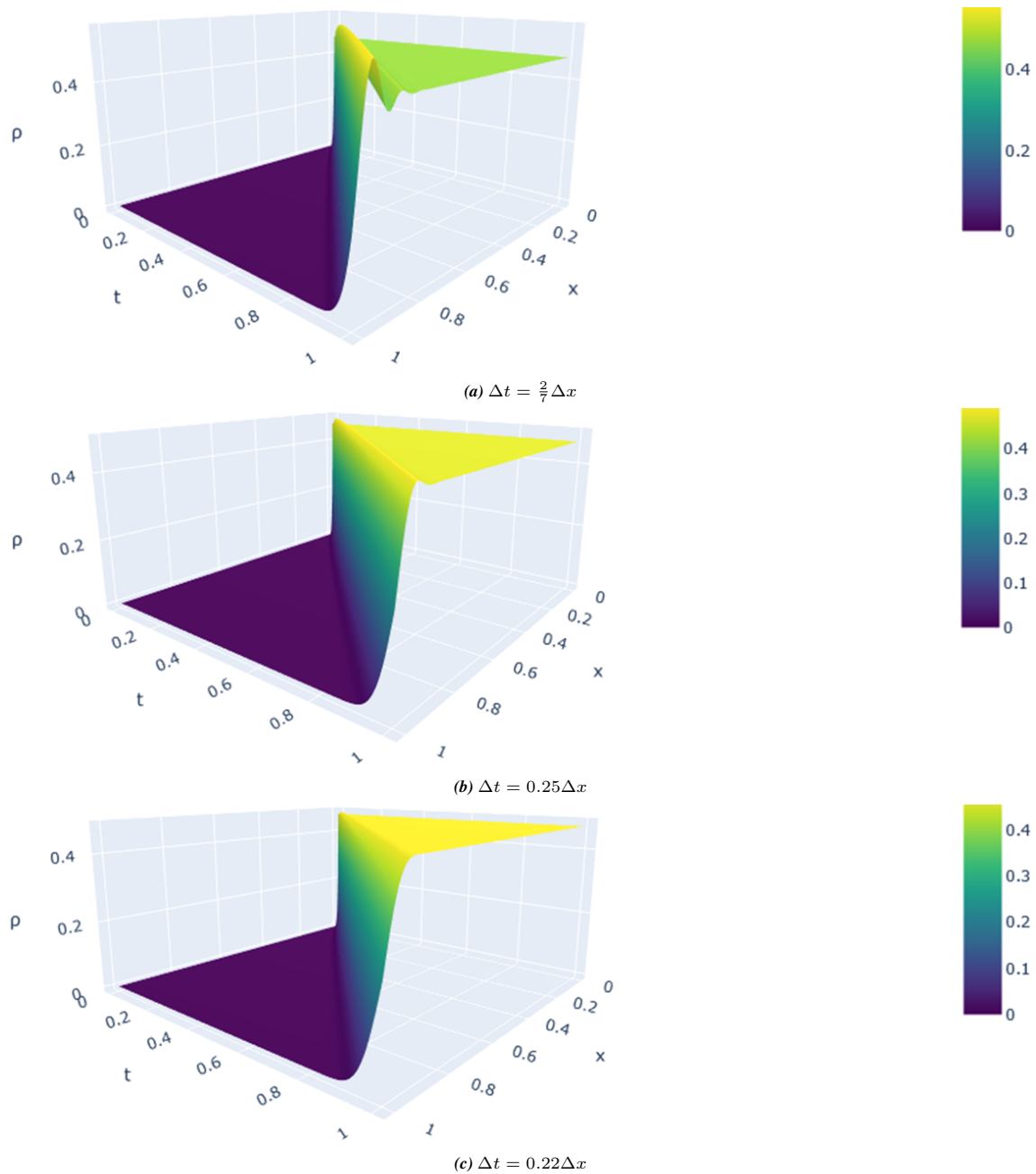
Figure 3. The density surface plot for first phase using upwind with double time filter in equation (26) of Algorithm 4.1 and different choices of \Delta t .
