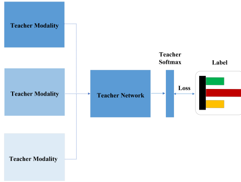
(c) Cross-model distillation with multi-teacher models using various modality data [42].
