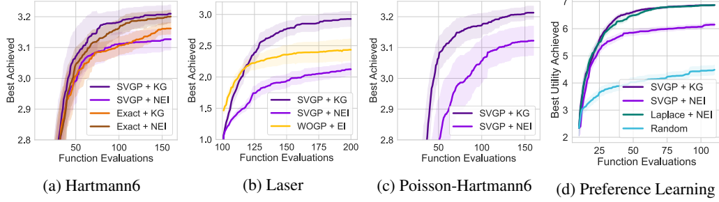
Figure 3: (a) Hartmann6 test problem with one constraint. Here, SVGPs with noisy expected improvement (qNEI) and KG match the performance of exact GPs with qNEI and qKG. (b) Free electron laser problem from McIntire et al. [51]; SVGPs with knowledge gradient outperforming weighted sparse GPs. (c) Constrained Hartmann6 test problem with count responses (Poisson likelihood). Only SVGPs can be used here, and qKG outperforms qNEI. (d) Preference learning; SVGPs with qKG are similar to Laplace approximations with NEI, and outperform qNEI with SVGPs.
