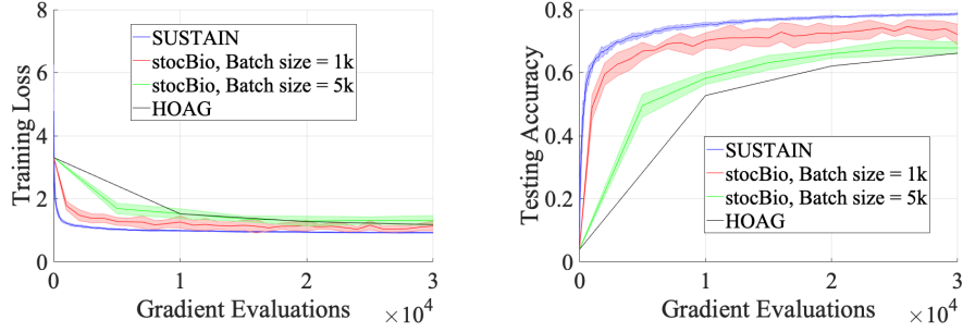
Figure 1: Hyperparameter optimization: Data hyper-cleaning task on the FashionMNIST dataset. We plot the training loss and testing accuracy against the number of gradients evaluated with corruption rate p = 0.3 .
