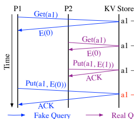
Figure 4: Correctness violation in one-layer approach.
