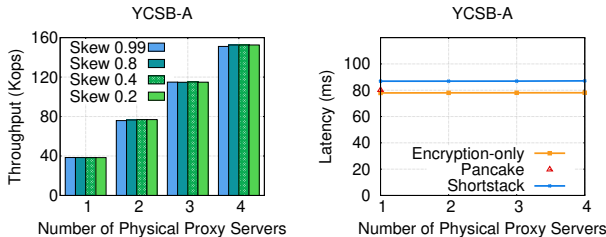
(a) SHORTSTACK throughput is unaffected by access skew.
