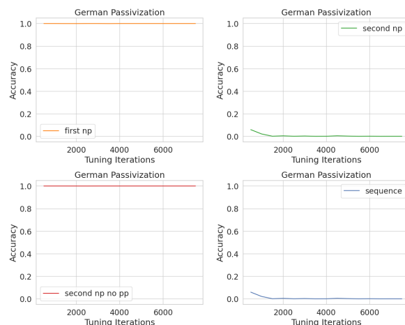
Figure 8: Learning curves displaying alternative accuracy metrics for mT5 on German passivization. We present the accuracy of the model in properly moving the object NP to the start of the sentence (top left), moving the subject NP after the auxiliary verb (top right), moving the subject NP after the auxiliary verb with or without its attached PP (bottom left), and the full sequence accuracy (bottom right).
