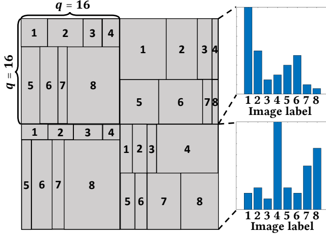
Fig. 9: Image formation in spatial multiplexing mode: The display is divided to hogels of size q \times q = 16 \times 16 pixels, and the area of each hogel is divided according to the desired energy distribution in this spatial position. e.g. if 25% of the hogel energy should be sent to direction 1, then 25% of the hogel area display slope \theta^1 . For example we demonstrate four hogels out of the entire display. On the right side we present the histogram of energies for the 8 different views (vector e(\vec{x}) ), and how each hogel area is divided displaying different slopes, hence sending different intensities at different directions. The numbers correspond to the different generated images, and image 8 acts as a residual image.
