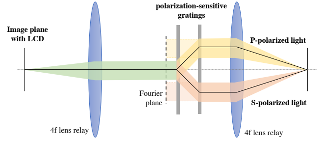
Fig. 3: Tilting rays by Fourier shifting: We use two polarization-sensitive gratings to shift the rays in the Fourier-plane, which introduces a tilt after the second lens. The colors, yellow and orange, show the two different polarization states and the paths they take after the grating layers. The shaded colors show the virtual path from which each polarized state appears to originate. The spacing between the gratings controls the tilts the rays experience. The LCD at the input image plane selects a polarization state, and this polarization leads to an independent tilt of light at each pixel.
