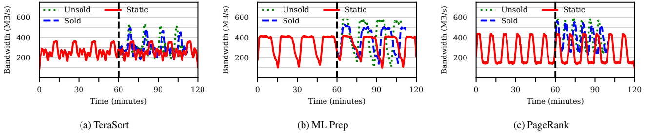
Figure 18: Performance benefits of storage harvesting for harvest VMs.
