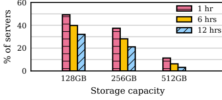
Figure 5: The availability of unallocated storage for harvesting.
