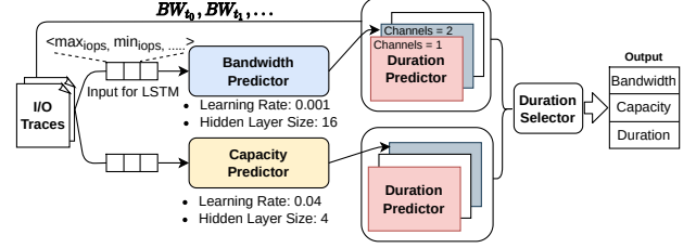
Figure 13: The workflow of the predictors used in BlockFlex.
