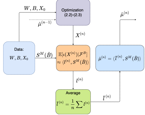
Figure 1. Flowchart of one iteration in the Sig-DFP Algorithm. Input: idiosyncratic noise W , common noise B , initial position X_0 and measure flow \hat{\mu}^{(n-1)} from the last iteration. Output: measure flow \hat{\mu}^{(n)} for the next iteration.
