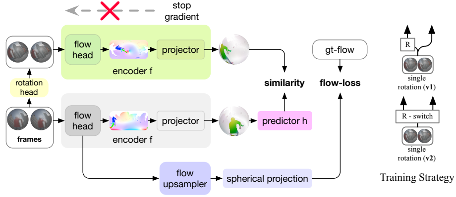
Fig. 1. Siamese Representation Learning for Omnidirectional Flow (SLOF). Pairs of frame sequence (w/ and w/o random rotation) are passed as inputs to encoder f (RAFT as a flow head backbone and a standard convolutional projector layer). A predictor layer h is an MLP layer. The entire framework is trained by fusing the pre-training and fine-tuning stage to combine the similarity and flow-loss in a single stage. The model maximizes the similarity between latent representations of flow information from two streams and minimizes the flow loss. Training Strategy (right): Here two different arrows( left, right ) represent siamese streams or input pathways to our model. v1 and v2 (either of the stream is subjected to rotational augmentation) are similar strategies achieving overall better performance.
