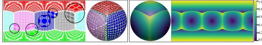
Fig. 7. Distortion density map. Illustrating different distortion intensity due to equirectangular projections. Left: upper (red) and lower (green) part of projections shows higher distortion in central part where as the equatorial region (cyan, pink, blue, gray) exhibit higher distortion rate away from the center of tangential plane. Right: shows the distortion density from (0, 1). This distortion density map is used to evaluate the distortion aware EPE ( EPE_d ). Note: Each circle patch in left spherical projection have same area.
