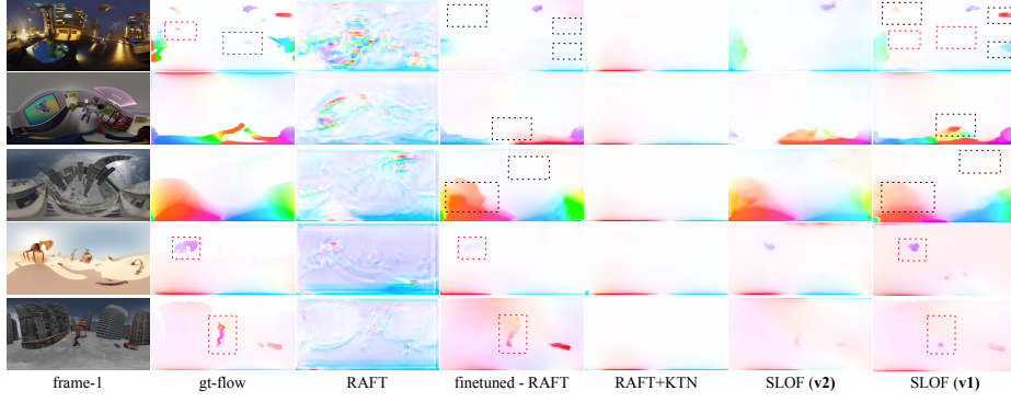
Fig. 6. Qualitative results on FLOW360 test set. Qualitative results show our best model SLOF(v1) shows better results compared to fine-tuned RAFT trained with policy explained in [61]. The dotted (black) rectangle indicates the comparative improvements of our model over fine-tuned RAFT. RAFT+KTN method fails to predict flow-field correctly; instead, it only predicts shallow flow fields from camera motion. The weakness of our model can be seen on dotted (red) rectangle where smaller motion segments are missing. Note: Flows information is clipped for better visualization.
