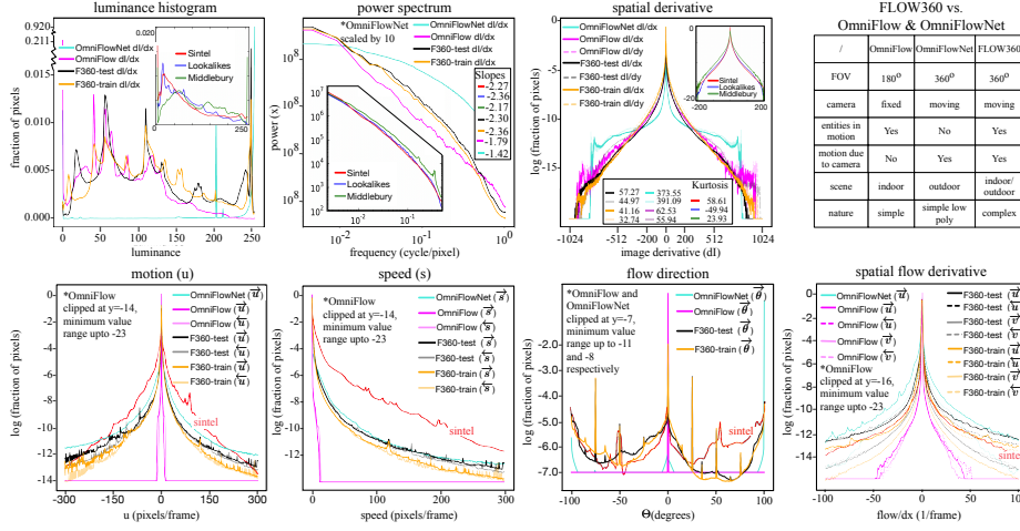
Fig. 5. Comparison of frames and flow statistics. Top row represents the frames statistics and comparison with Sintel, Lookalikes, Middlebury, OmniFlow [52] and OmniFlowNet [3]. Bottom row represents flow statistics and comparison with Sintel (red), OmniFlow (magenta) and OmniFlowNet (turquoise). The table on the top-right shows a brief comparison of OmniFlow & OmniFlowNet with FLOW360 dataset. Note: ( \rightarrow , \leftarrow ) represents forward and backward flow fields, respectively.
