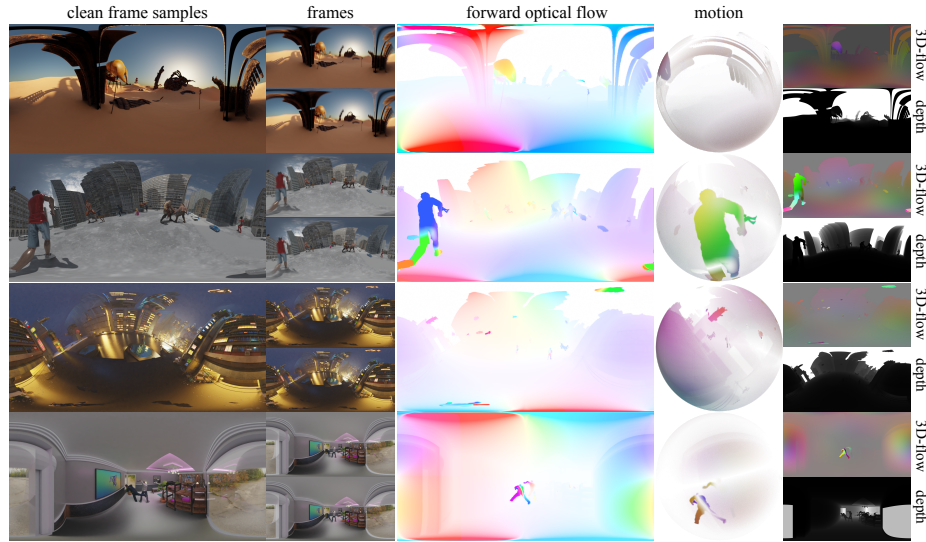
Fig. 2. The FLOW360 Dataset. Sample frames (first and second column, respectively) from some of the videos with corresponding forward optical flow and dynamic depth information. Motion in 3D Sphere (fourth column) is computed by transforming the motion vectors from Equirectangular plane (\theta, \phi) to unit sphere f(x, y, z) . Motion in the sphere is represented in RGBA color notation. RGB color representation (as suggested in Middlebury [6]) is encoded using (x, y) components, and the alpha color is encoded from z of a unit sphere. RGB encoding (fifth column) is an RGB color map of flow in 3D space. Note: flow fields are clipped for better visualization.
