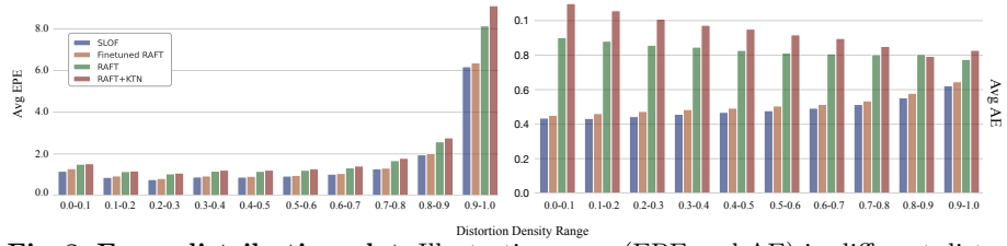
Fig. 8. Error distribution plot. Illustrating error (EPE and AE) in different distortion density ranges. SLOF relatively performs better in all distortion density ranges.
