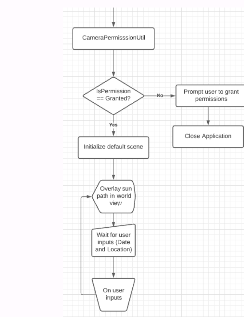
Figure 5: Water AR app flow chart
