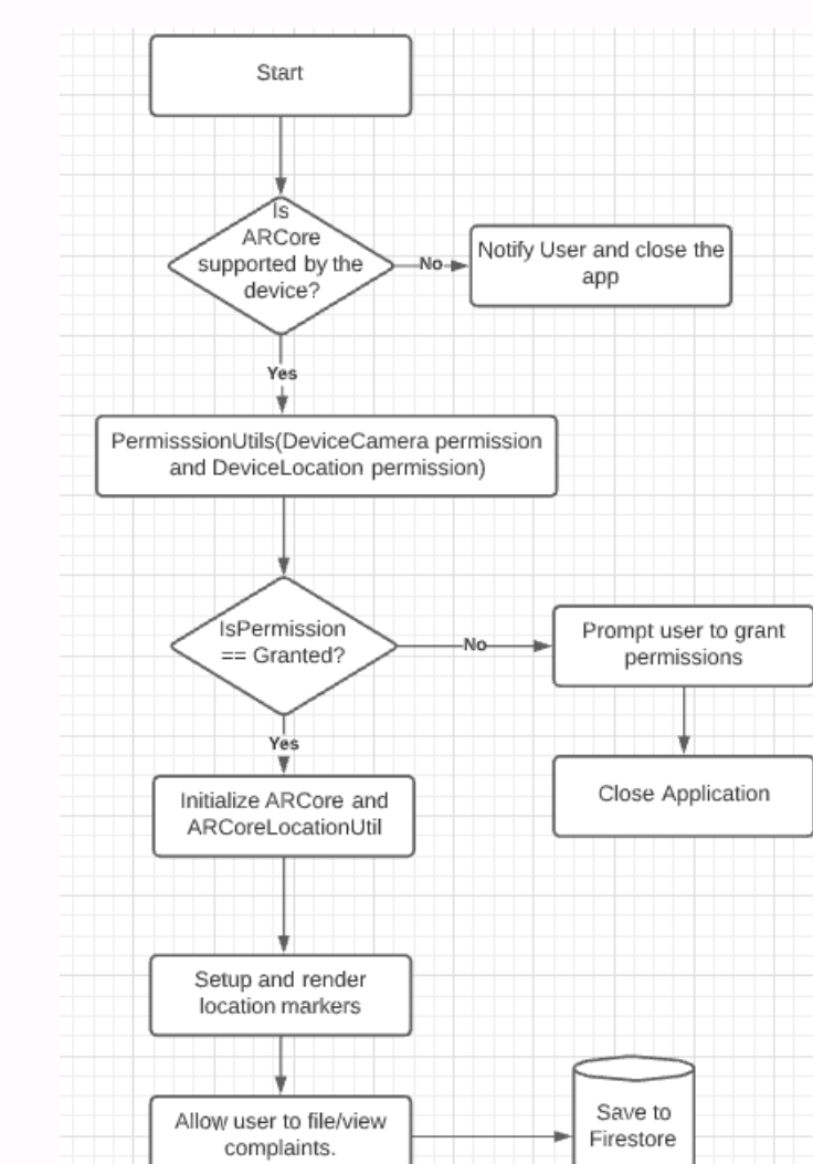
Figure 4: Water AR app flow chart
