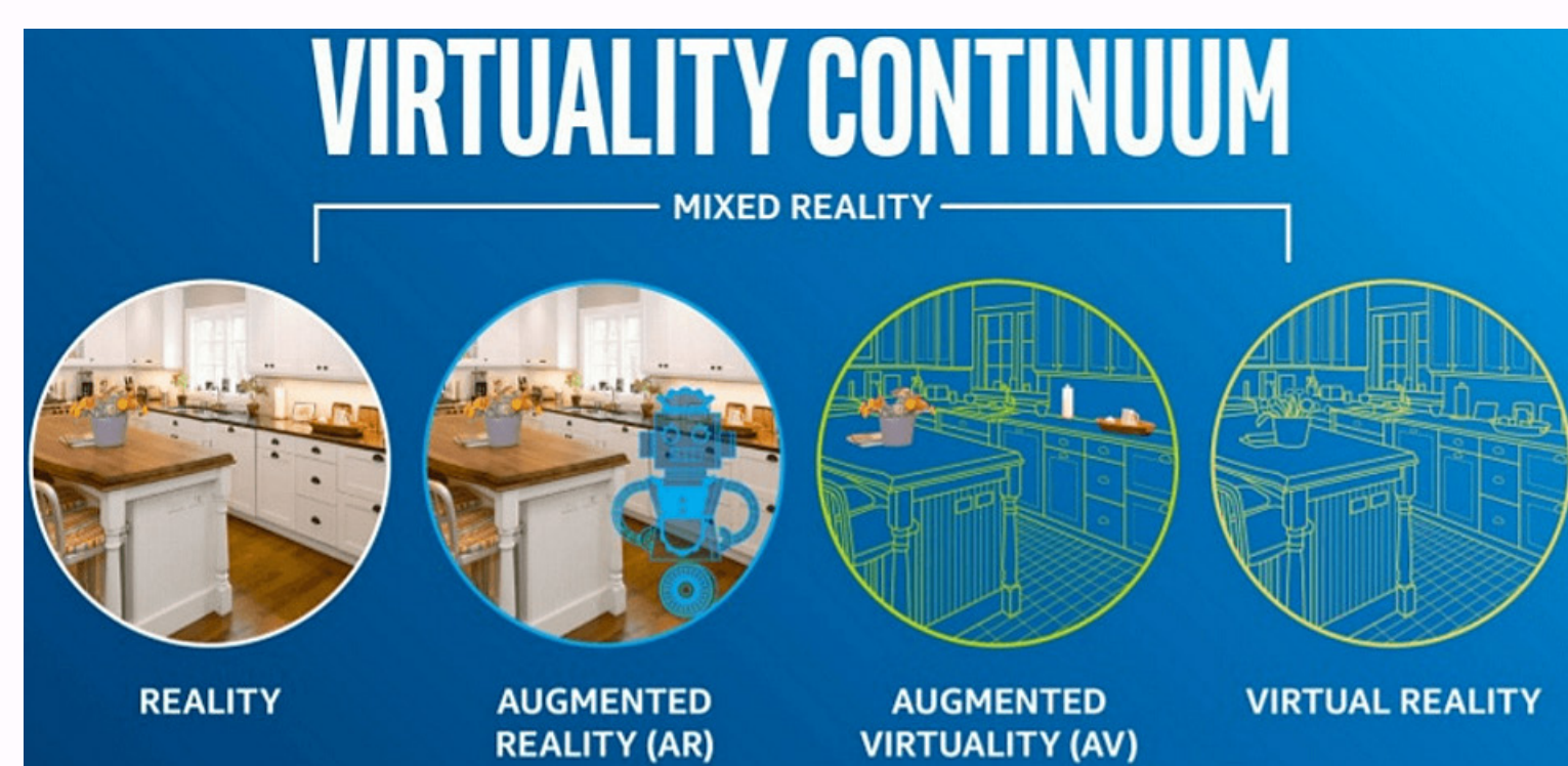
Figure 3: Reality-virtuality continuum
