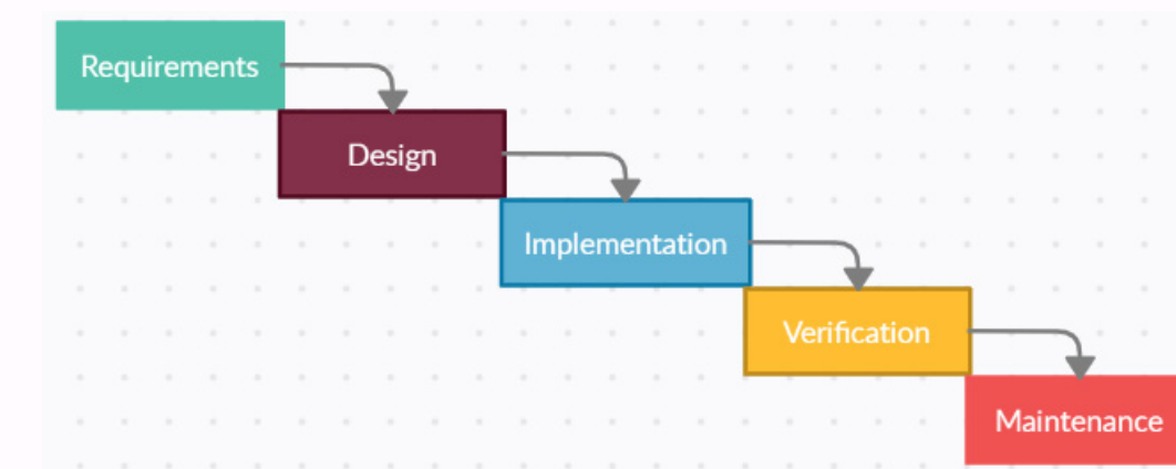
Figure 7: Waterfall Model
