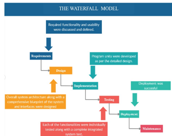
Figure 7. Waterfall Model.
