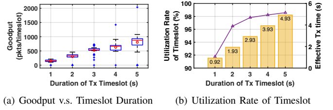
(a) Goodput v.s. Timeslot Duration (b) Utilization Rate of Timeslot Fig. 10. Goodput & Utilization Rate v.s. Timeslot Duration
