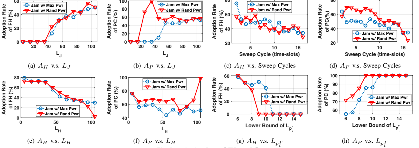
Fig. 7. Adoption Rate of FH and PC
