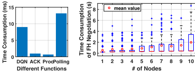
(a) Typical Functions (b) Time Consumption v.s. Network Size Fig. 9. Time Consumption
