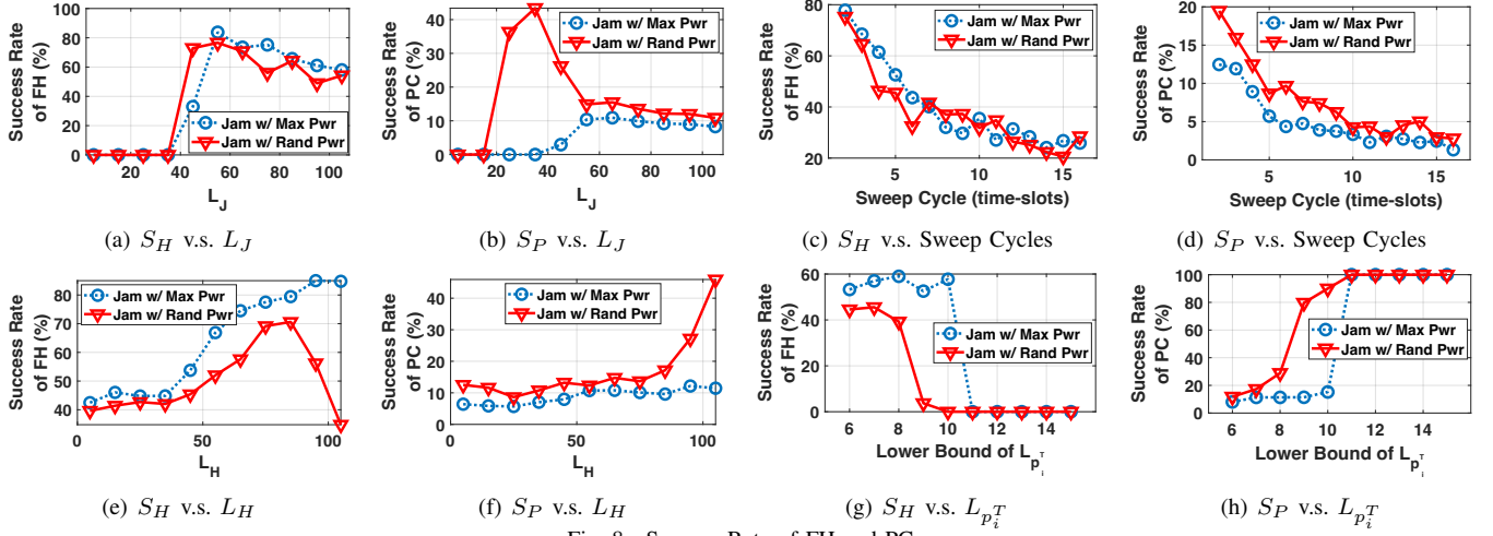
Fig. 8. Success Rate of FH and PC
