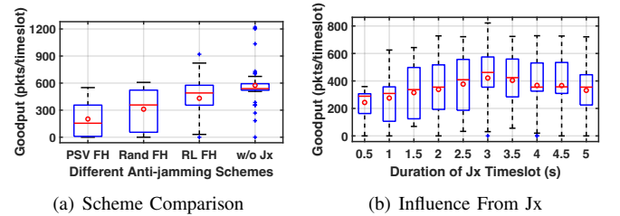
(a) Scheme Comparison (b) Influence From Jx Fig. 11. Schemes Comparison & Analysis
