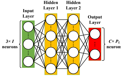
Fig. 4. Neural Network Architecture of DQN Fig. 5. Experiment Setting
