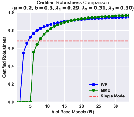
(a) [a, b] = [0.2, 0.3], \lambda_1 = 0.29, \lambda_2 = 0.31, \lambda_3 = 0.30 .
