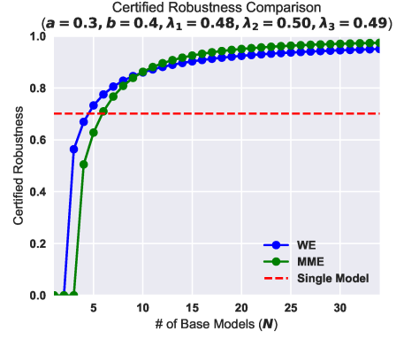
(b) [a, b] = [0.3, 0.4], \lambda_1 = 0.48, \lambda_2 = 0.50, \lambda_3 = 0.49 .
