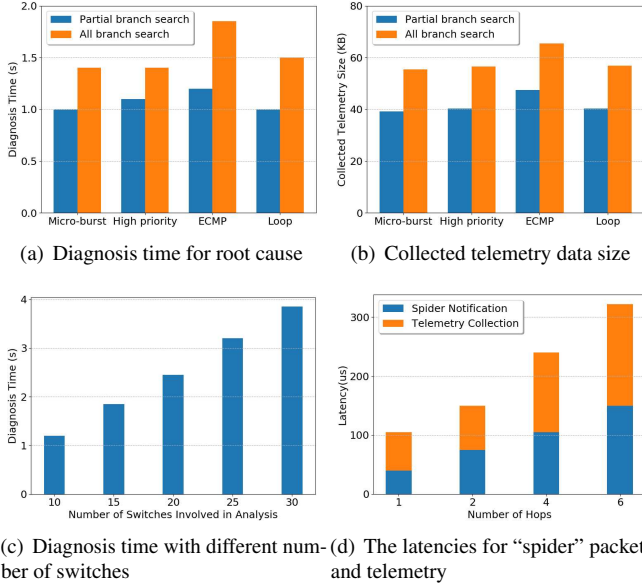
Figure 10: Branch-search metrics for SpiderMon
