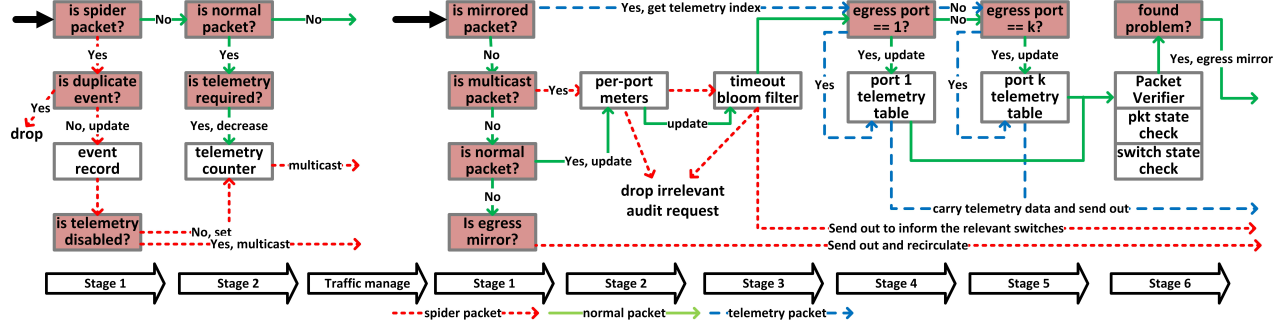
Figure 14: The placement of SpiderMon components on the switch stages
