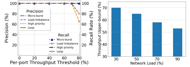
Figure 11: Throughput metrics for SpiderMon
